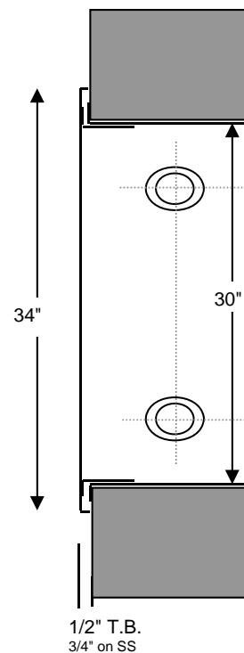
SIDE
