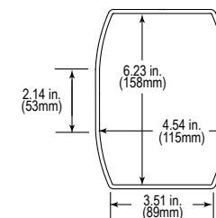
CENTER DIMENSIONS
